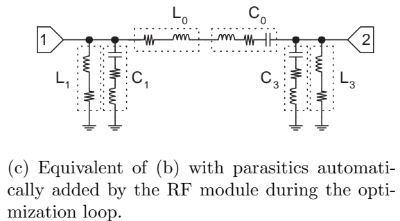
Figure 6.4: The Chebyshev band pass filter.
